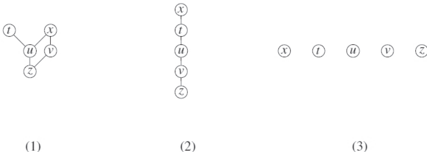
FIGURE 1. - Hasse diagrams of a poset (1), a chain (2) and an antichain (3)
