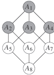
FIGURE 5. - Image of P under the map \varphi . In grey, deprived binary profiles
