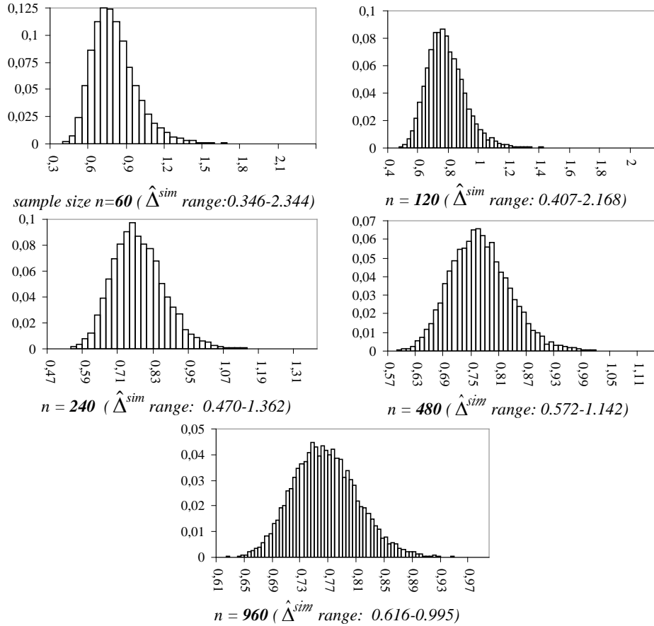
Figure 10. Simulated distributions of the s.m.d. \hat{\Delta}_n (by 10,000 samples, drawn from the Pareto ( x_0 = 2, \theta = 4 ))
