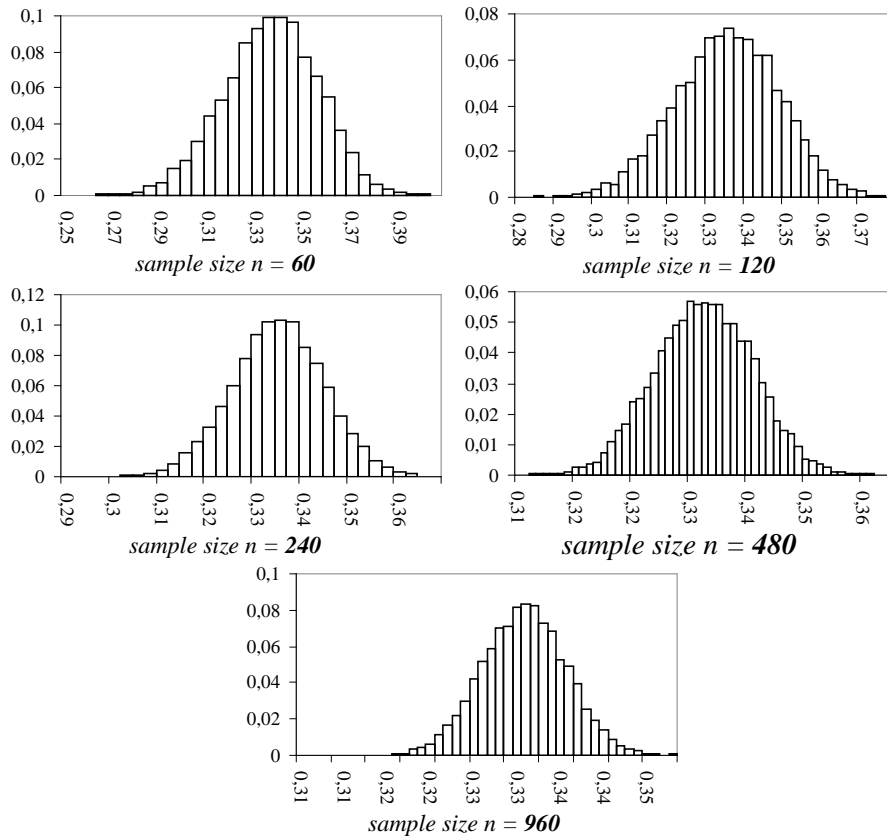
Figure 4. Simulated distribution of the s.m.d. \hat{\Delta}_n (by 10,000 samples, drawn from the Rectangular ( a=0, b=1 )).
