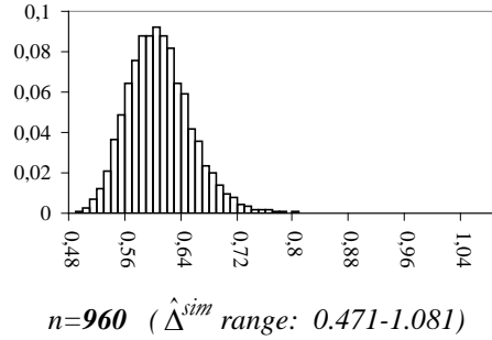
Figure 8. (continuation) Simulated distribution of the s.m.d. \hat{\Delta}_n (by 10,000 samples, drawn from the Pareto ( x_0=1, \theta=3 ))
