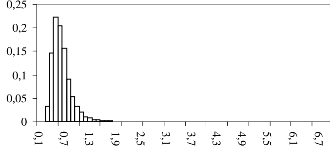
Figure 7. Simulated distribution of the s.m.d. \hat{\Delta}_n (by 10,000 samples, n=30 , drawn from the Pareto distribution with x_0 = 1 , \theta = 3 )
