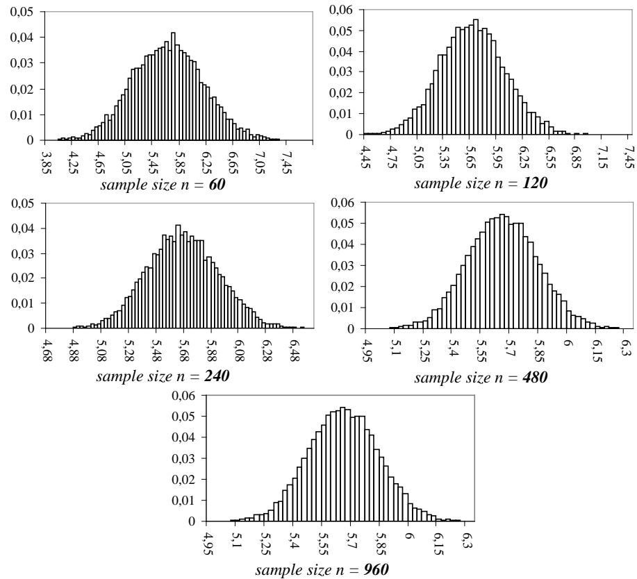
Figure 2. Simulated distribution of the s.m.d. \hat{\Delta} (by 10,000 samples, drawn from the \text{Normal}(\mu=0; \sigma=5) )
