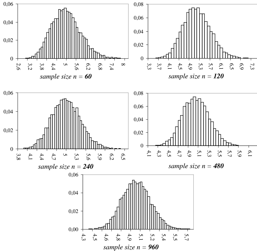
Figure 6. Simulated distribution of the s.m.d. \hat{\Delta}_n (by 10,000 samples, drawn from the Exponential, \theta = 0.2 )
