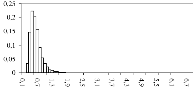
Figure 9. Simulated distribution of the s.m.d. \hat{\Delta}_n (by 10,000 samples, n=30 , drawn from the Pareto distribution with x_0 = 1 , \theta = 3 )
