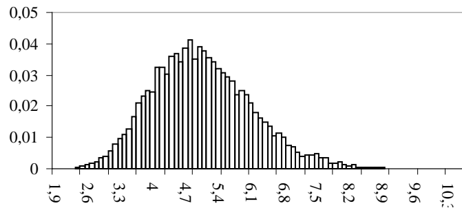
Figure 5. Simulated distribution of the s.m.d. \hat{\Delta}_n (by B=10,000 samples, n=30 , drawn from the Exponential distribution with \theta = 0.2 )
